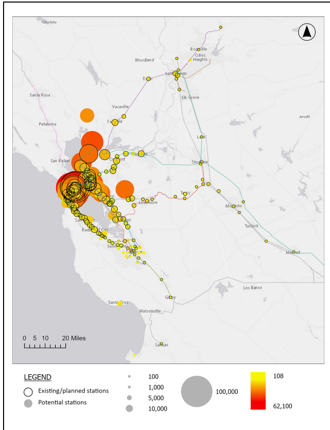
Figure 3. Transbay equity-weighted unmet rail potential (number of potential trips), 2040.
